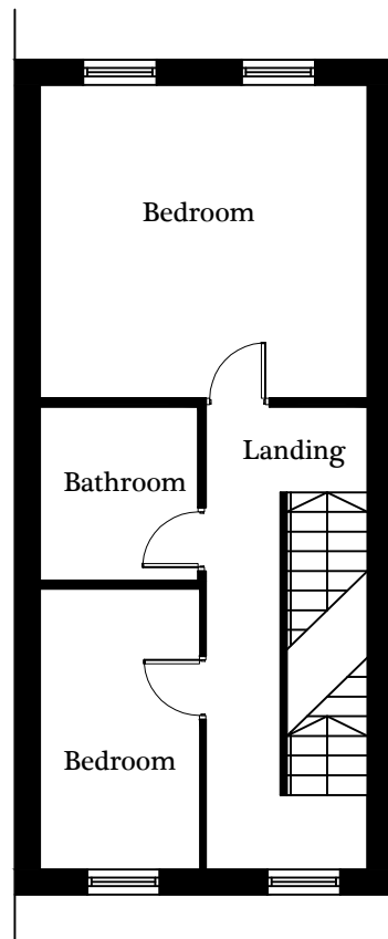
Existing First Floor Plan @ 1:100 Scale
