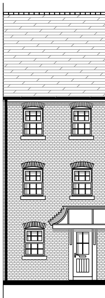
Existing Front Elevation @ 1:100 Scale
