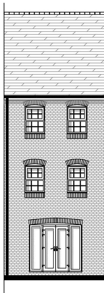
Existing Rear Elevation @ 1:100 Scale
