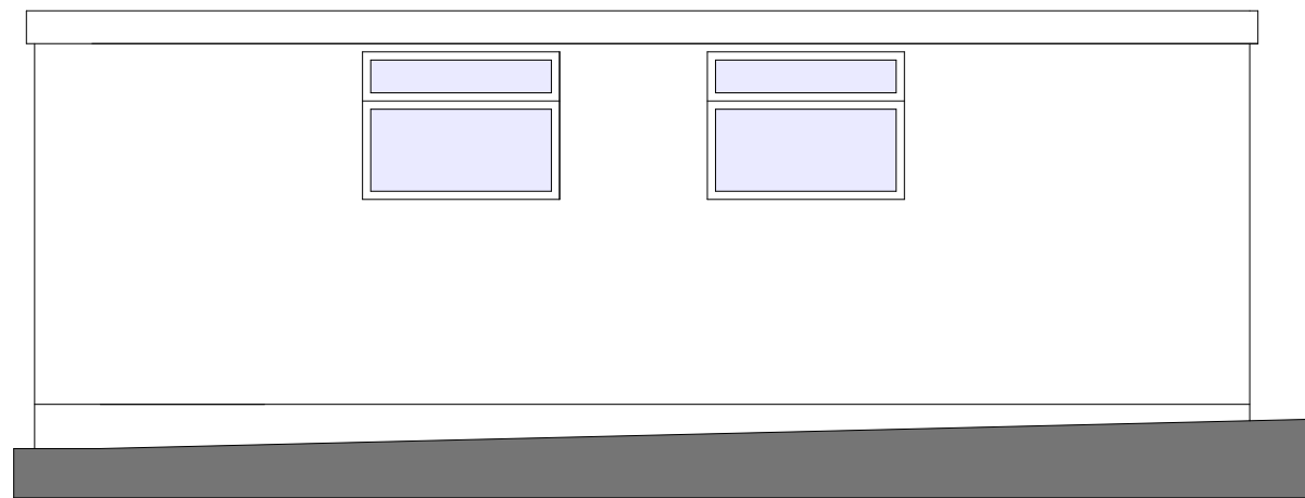
Proposed Side Elevation - facing fence
