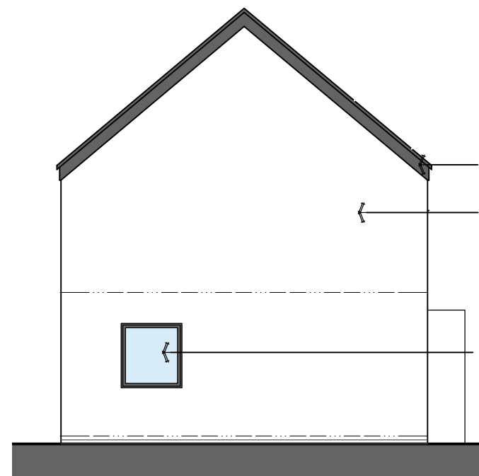
South elevation (Plot 1) 1:100 West elevation (Plots 3 & 4) 1:100
