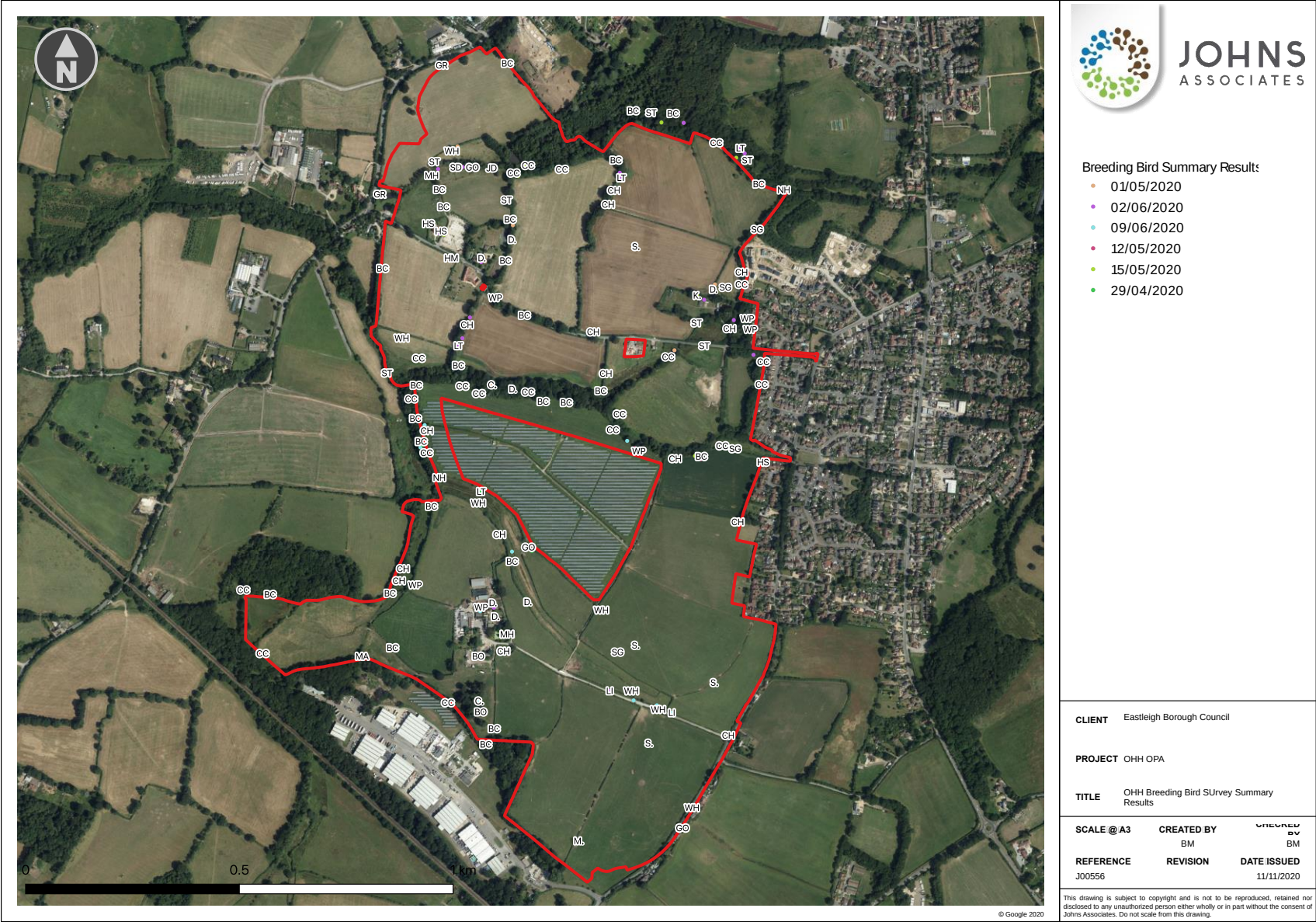
Figure 2 Breeding Bird Survey 2020 - Summary Results - All Species
