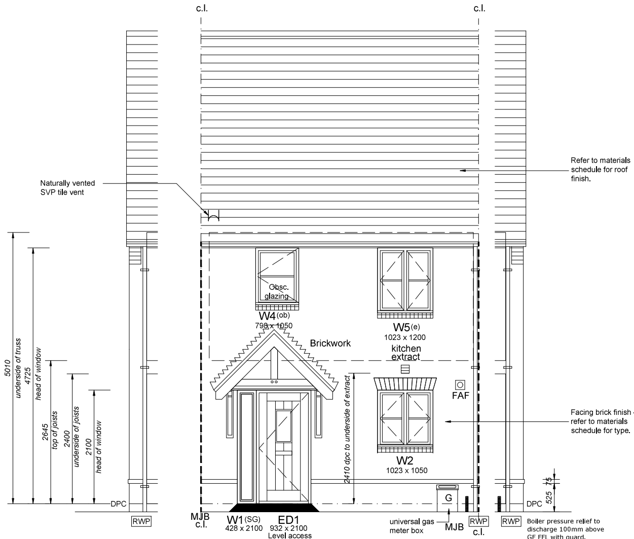
Front Elevation
