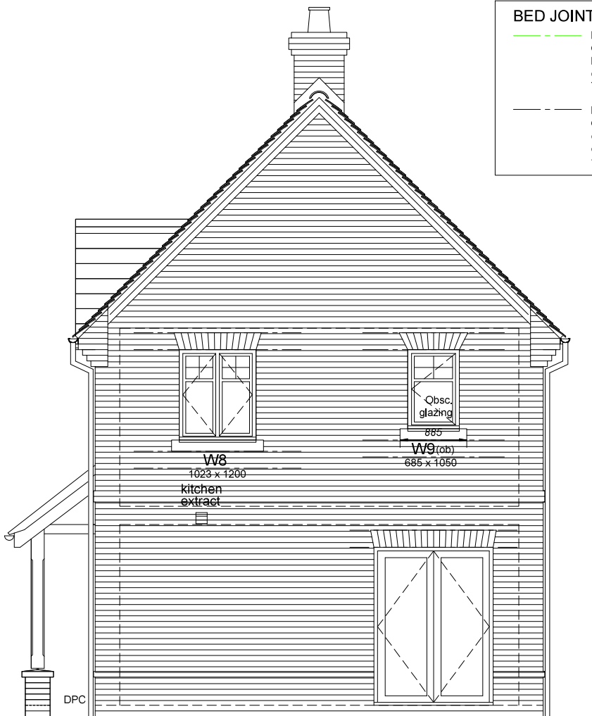
Side Elevation
