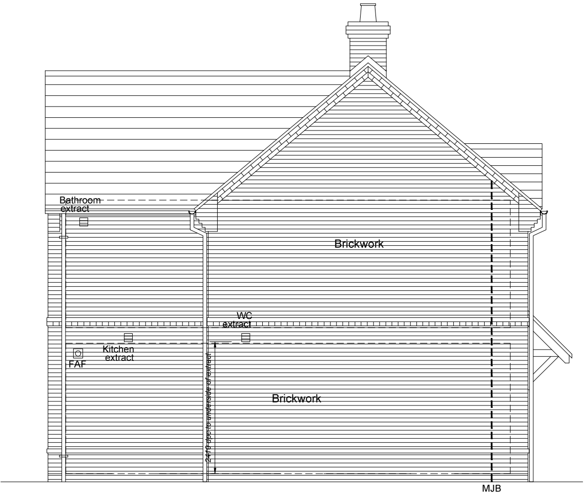
Side Elevation Plots AS 347
