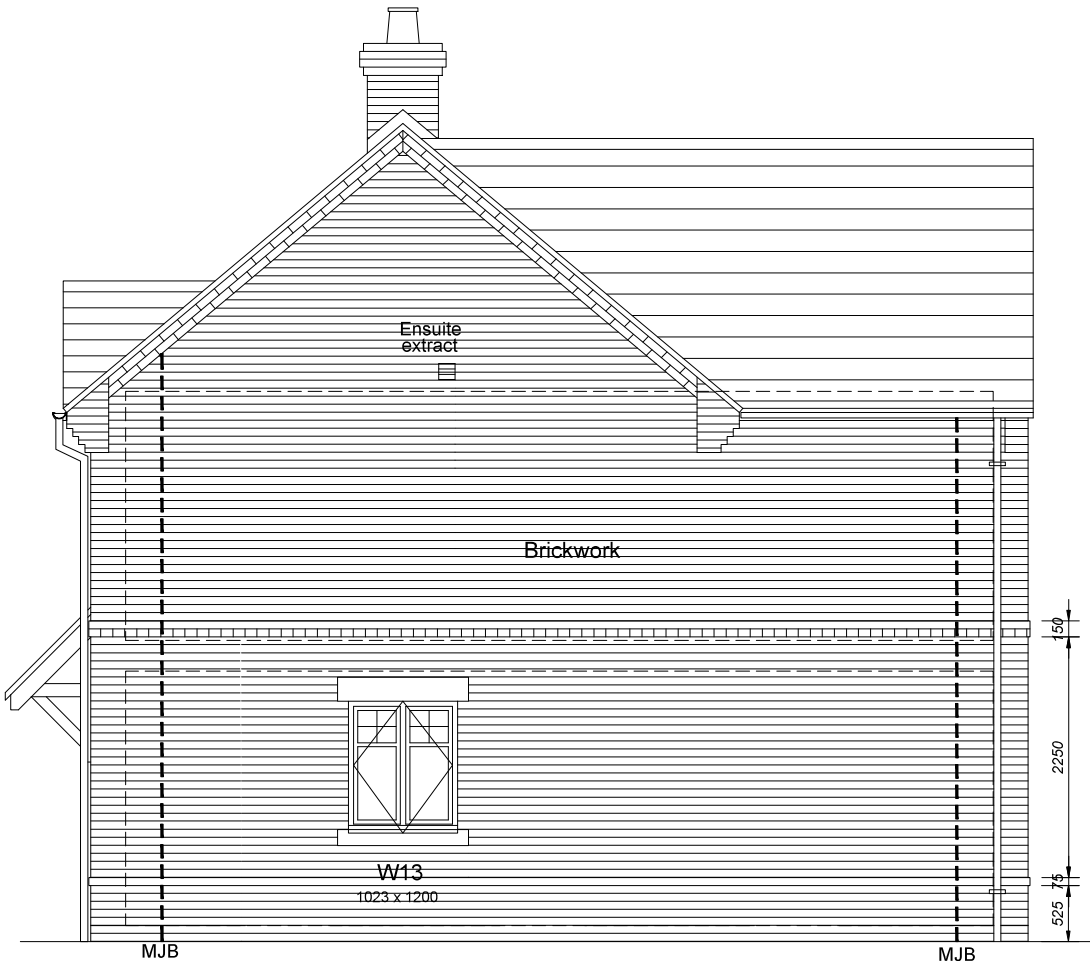
Side Elevation Plots AS 347
