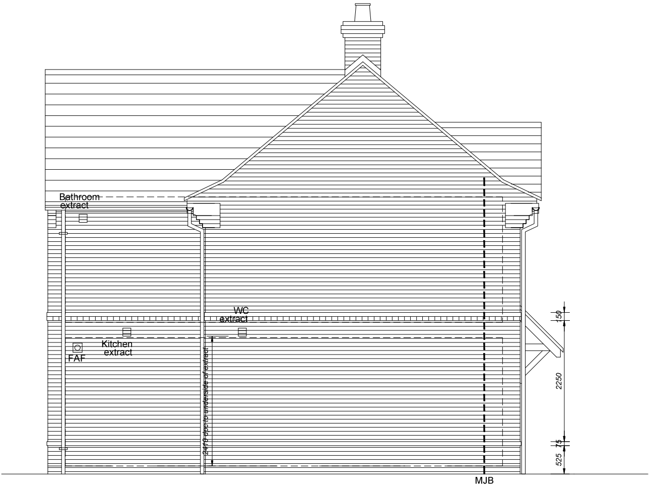
Side Elevation Plots OPP 334
