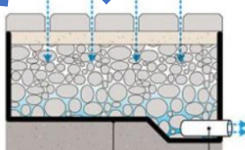
Permeable Paving
