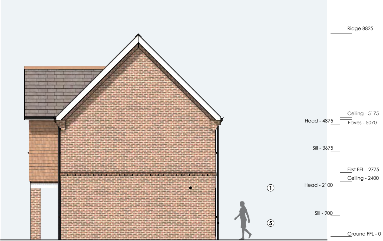
South Elevation - Side
