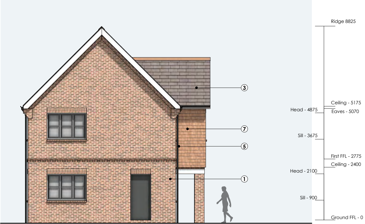
North Elevation - Side
