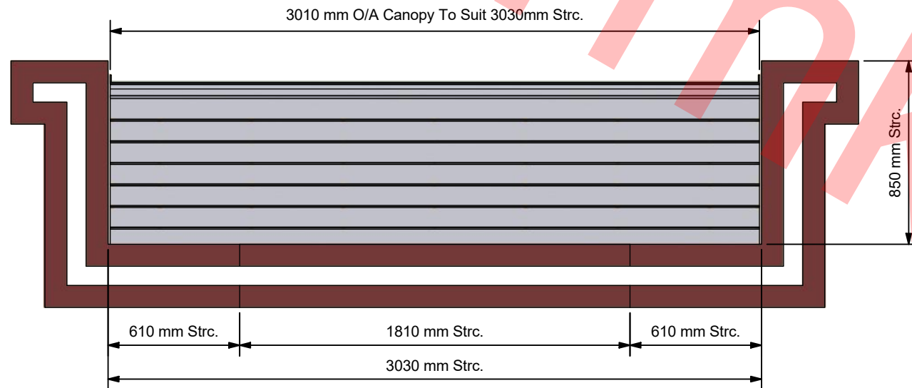
Reflected Plan Elevation (View From Beneath) ( 1 : 25 )
