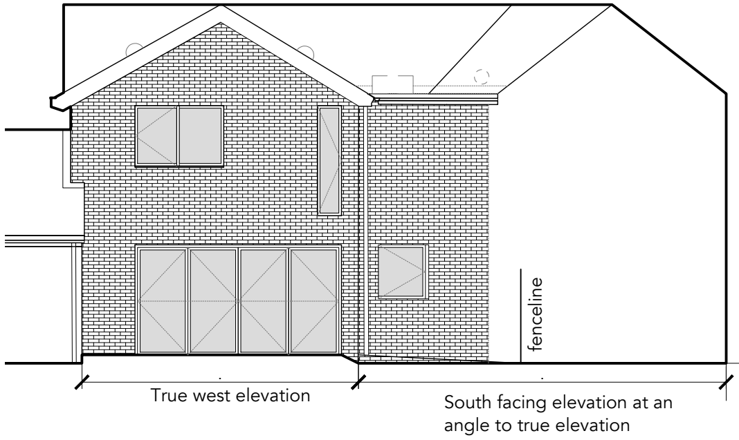
WEST ELEVATION 1:100 @ A3
