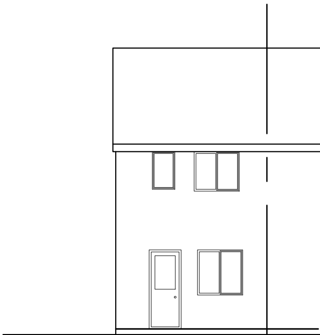
Rear Elevation.
