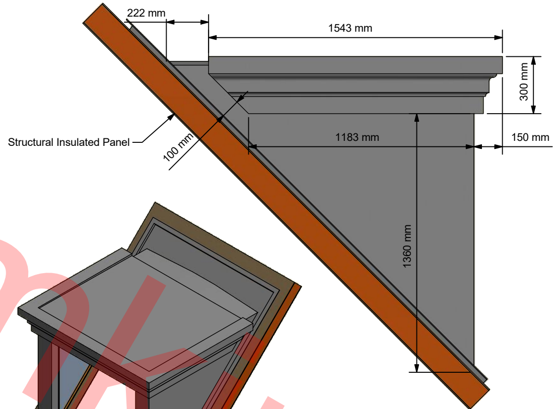
Side Elevation ( 1 : 20 )
