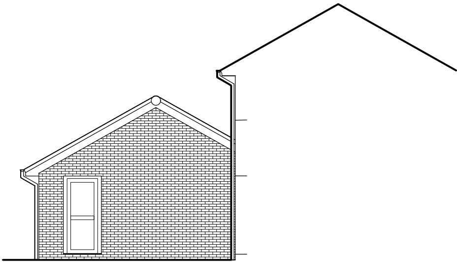
SOUTH ELEVATION 1:100 @ A3
