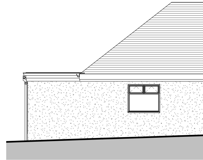
East as Existing 1:100
