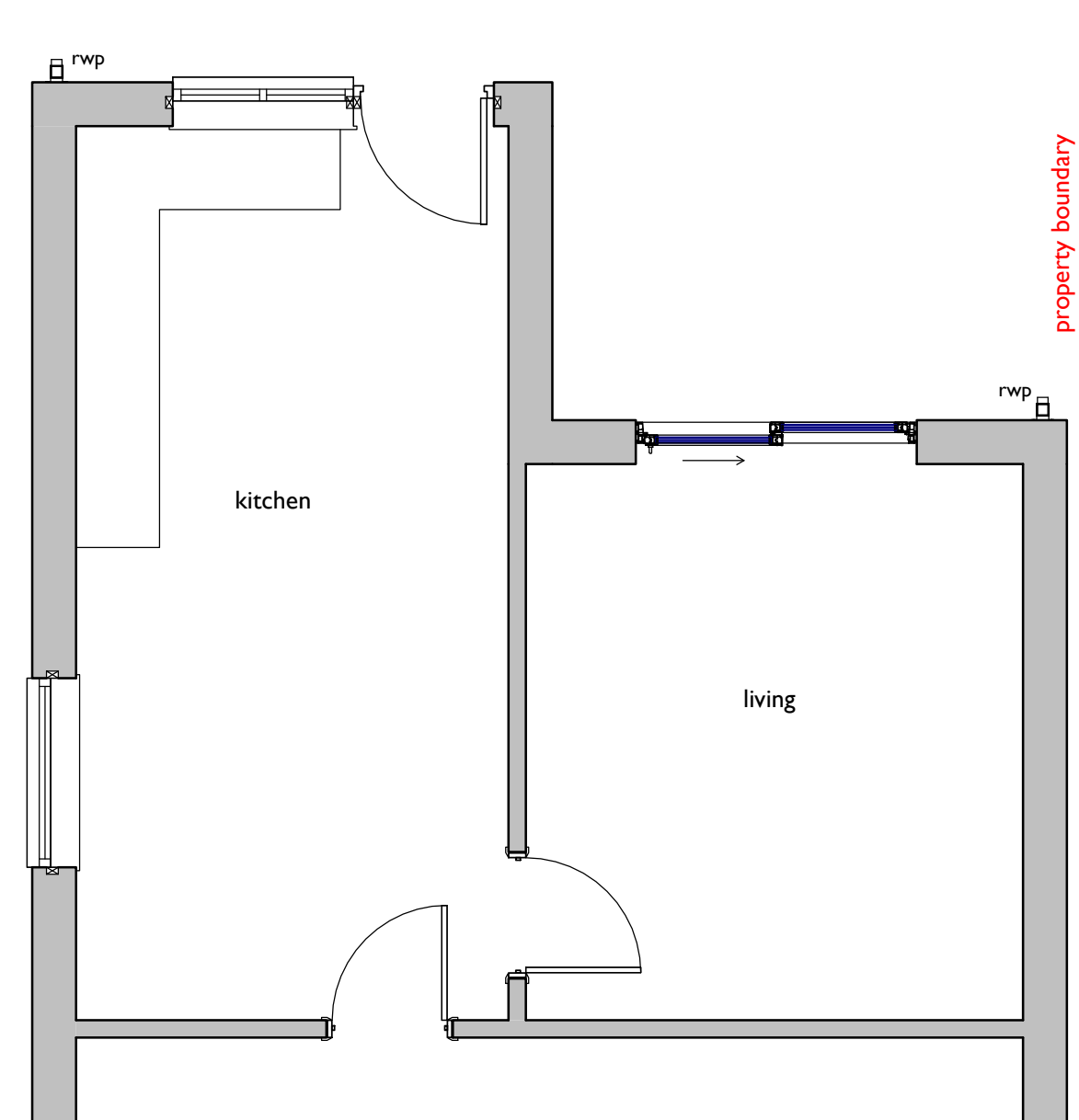
Ground as Existing 1:50
