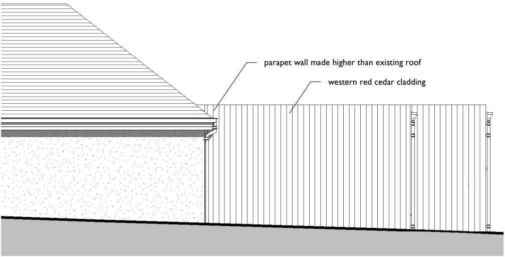
West as Proposed 1:100
