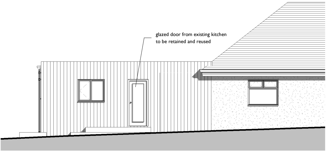
East as Proposed 1:100
