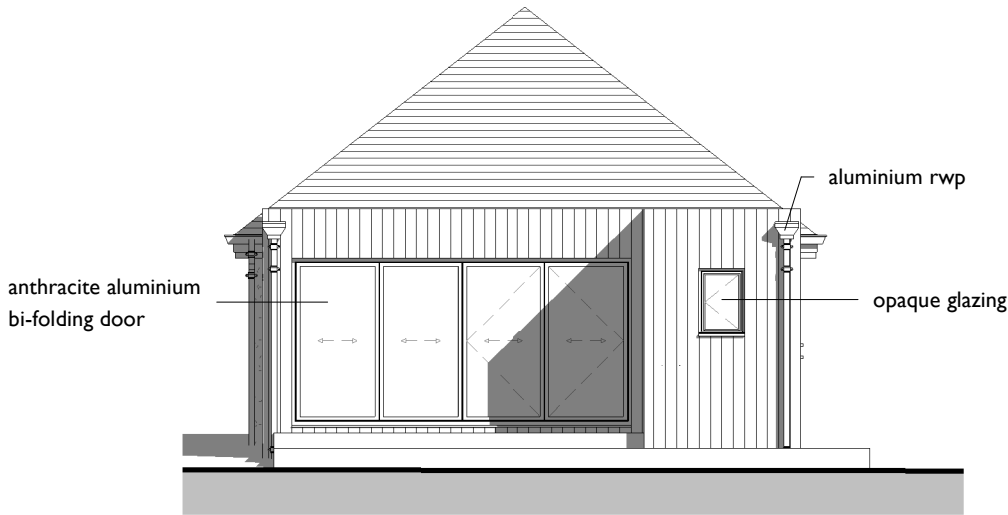
South as Proposed 1:100
