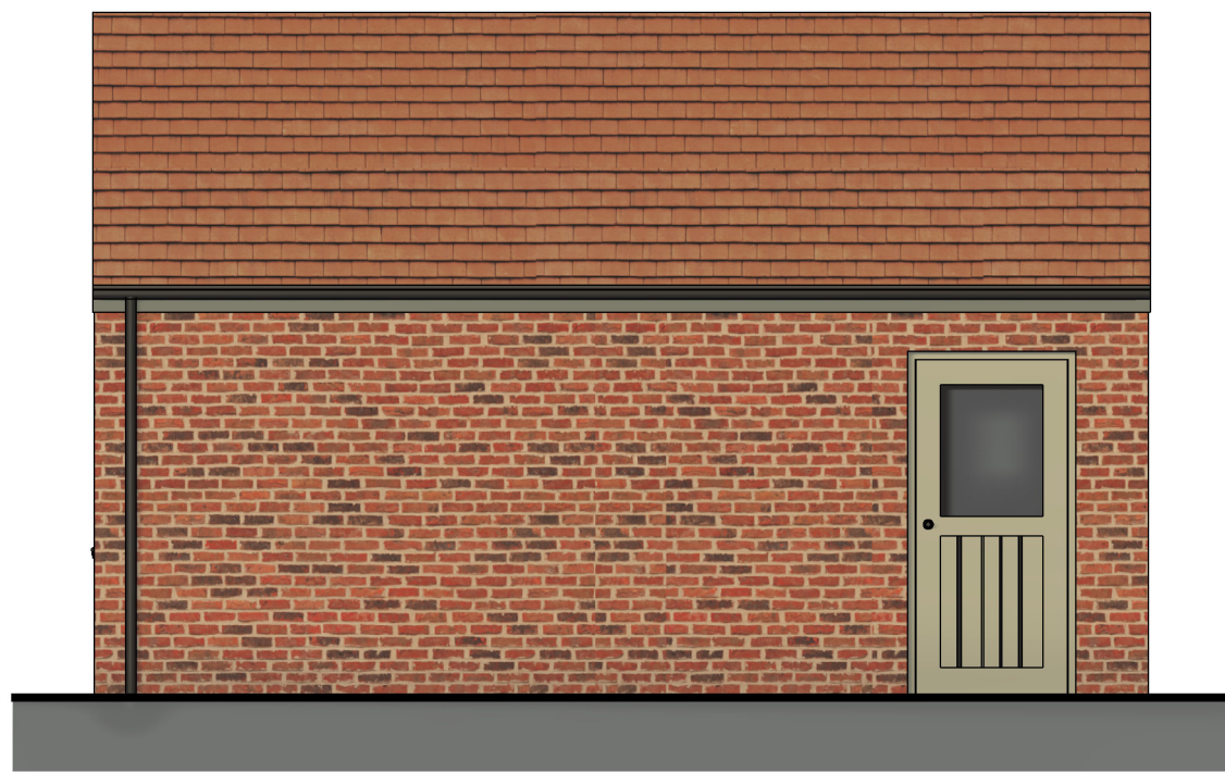
Side Elevation 2 1 : 50
