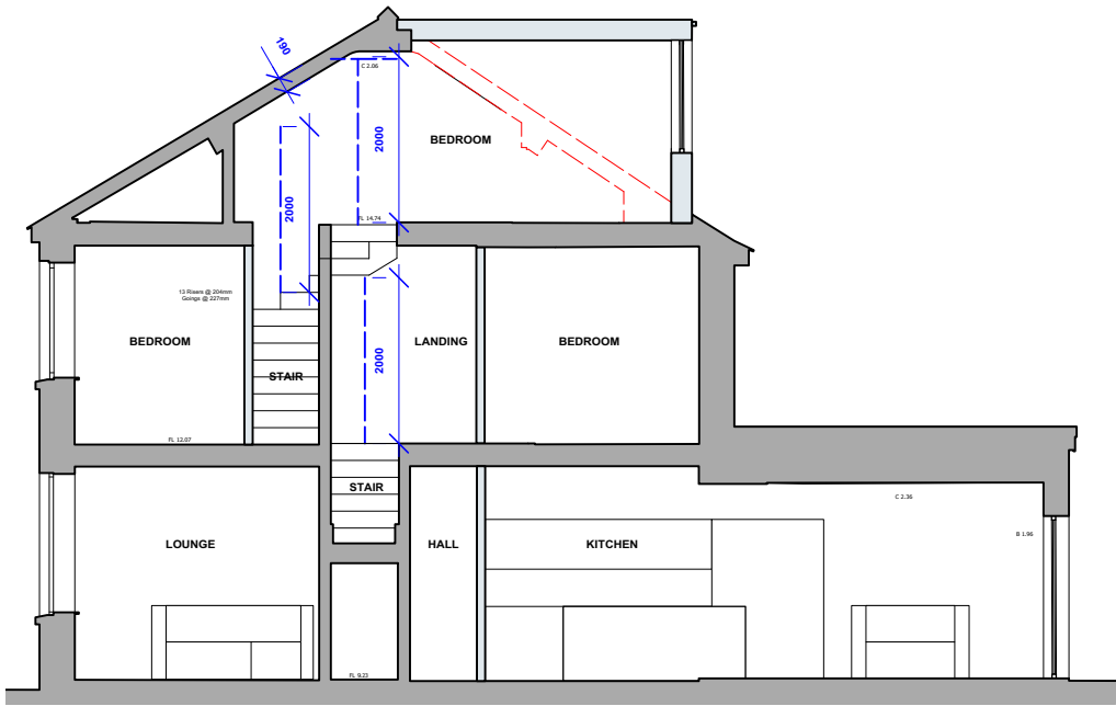
2 Section B-B
