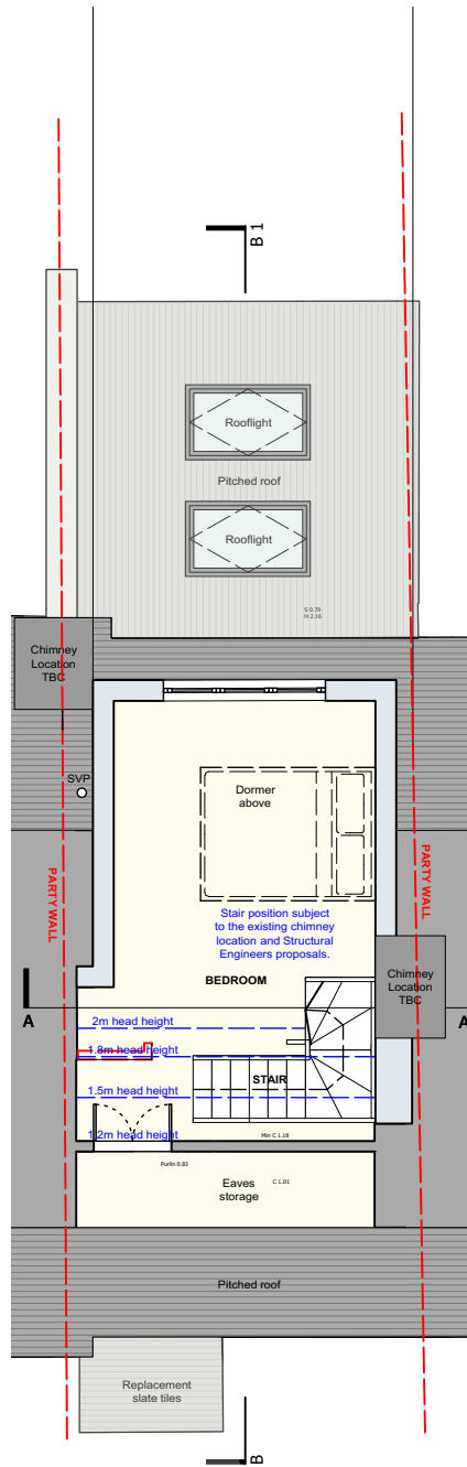
3 Second Floor Plan
