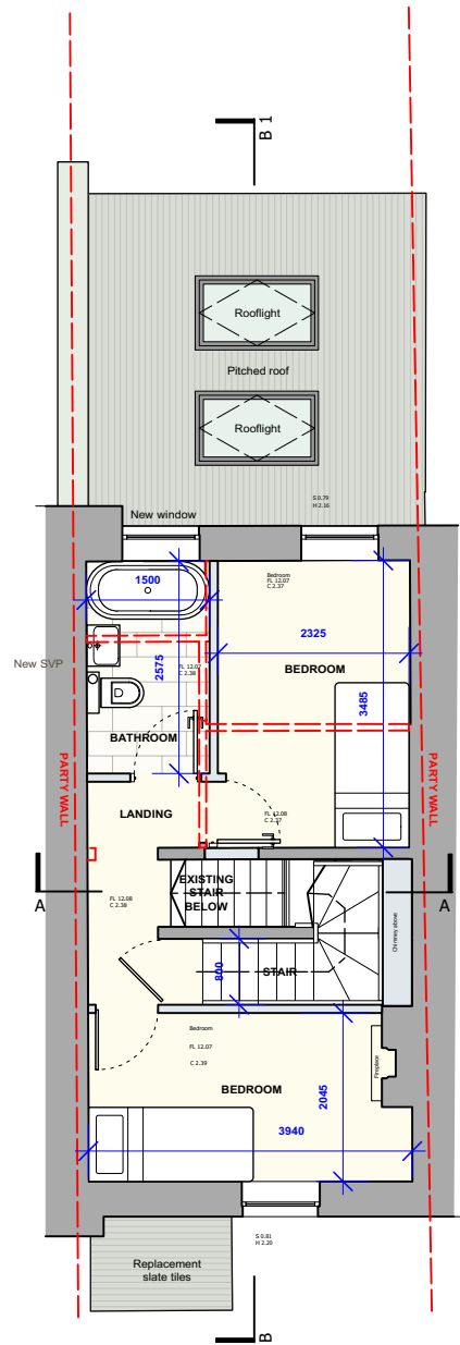
2 First Floor Plan
