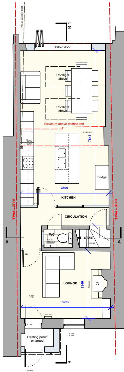
1 Ground Floor Plan
