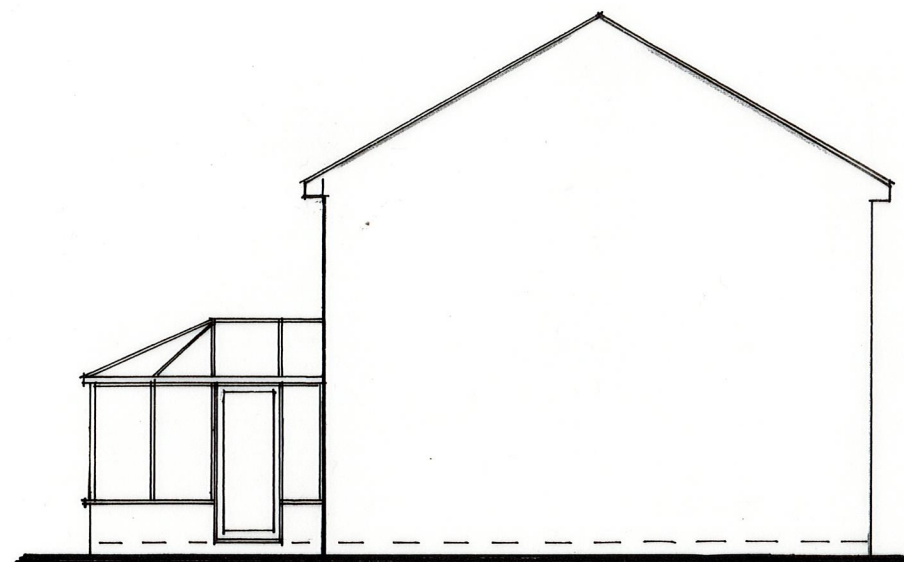
SIDE ELEVATION 1:100
