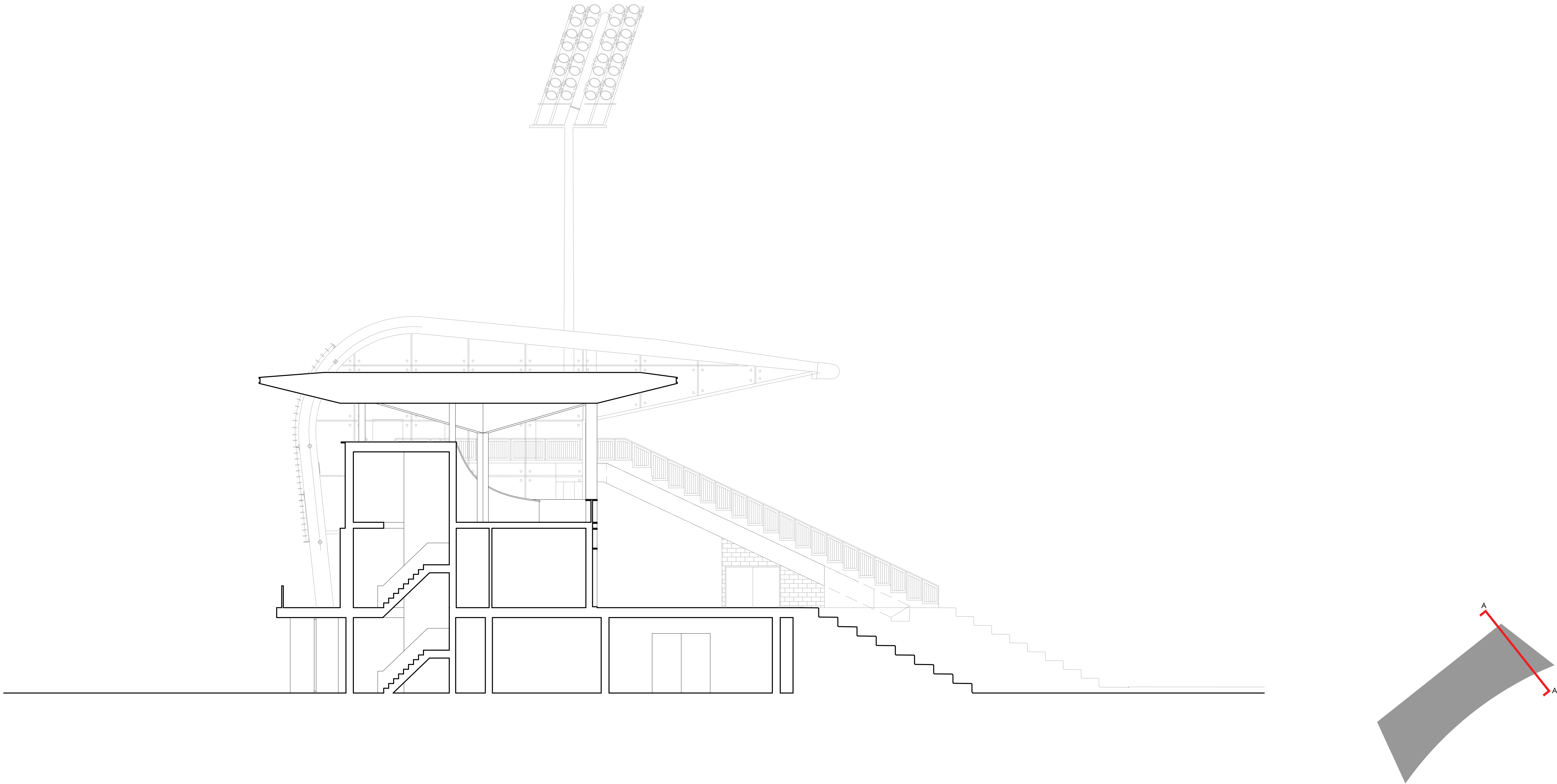
SECTION AA
