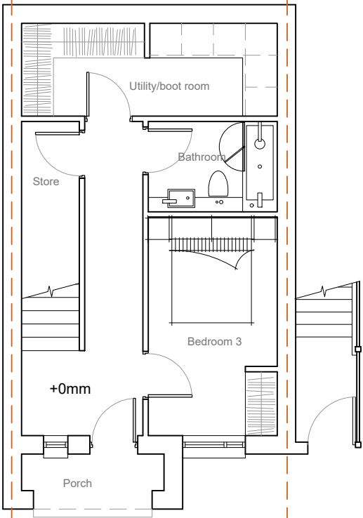
GROUND FLOOR 37.4sq.m. TOTAL 138.4sq.m. (1490sq.ft.)
