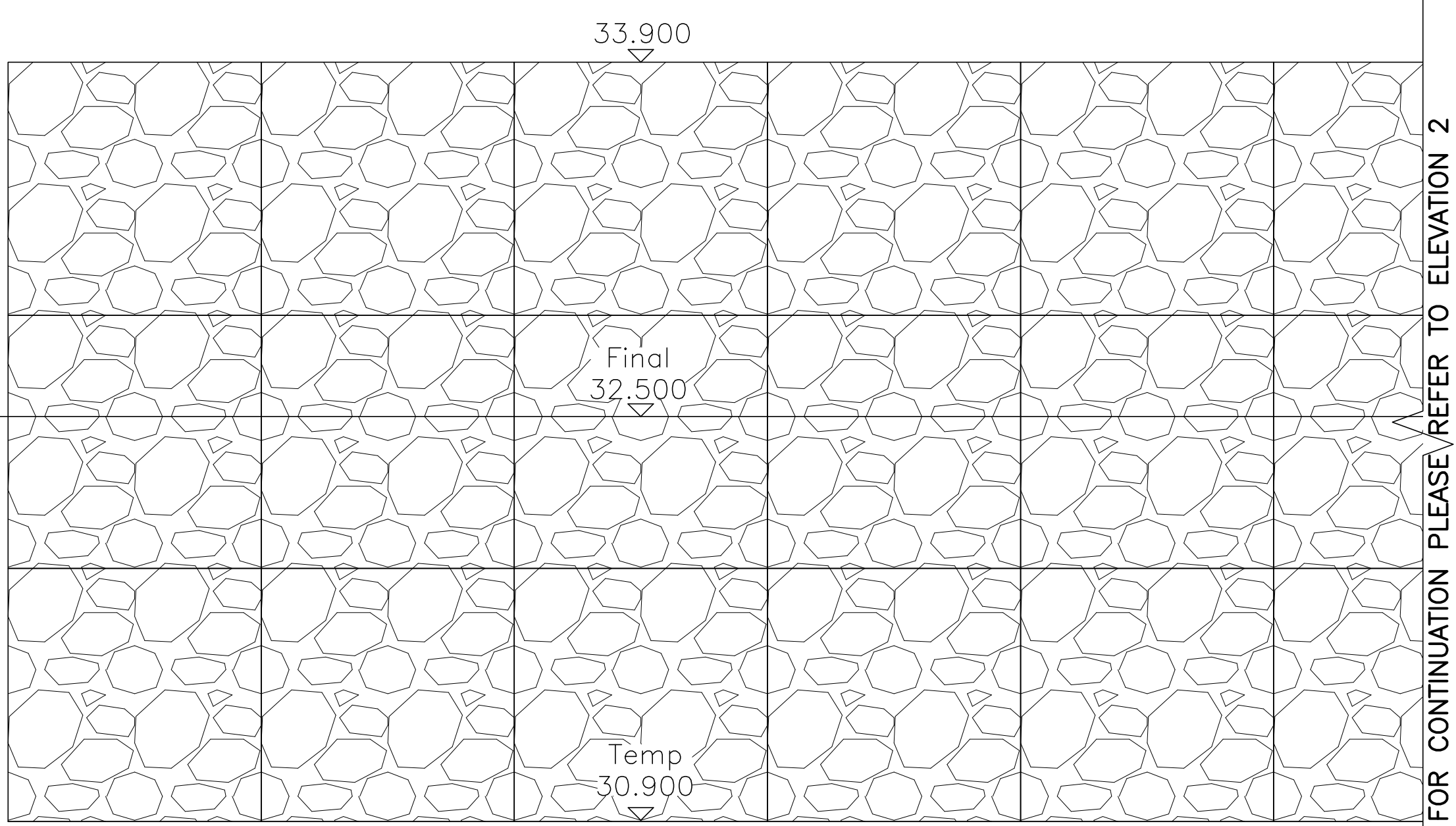
WALL 3/ELEVATION 3 Woven Gabion Retaining Wall (1:20)
