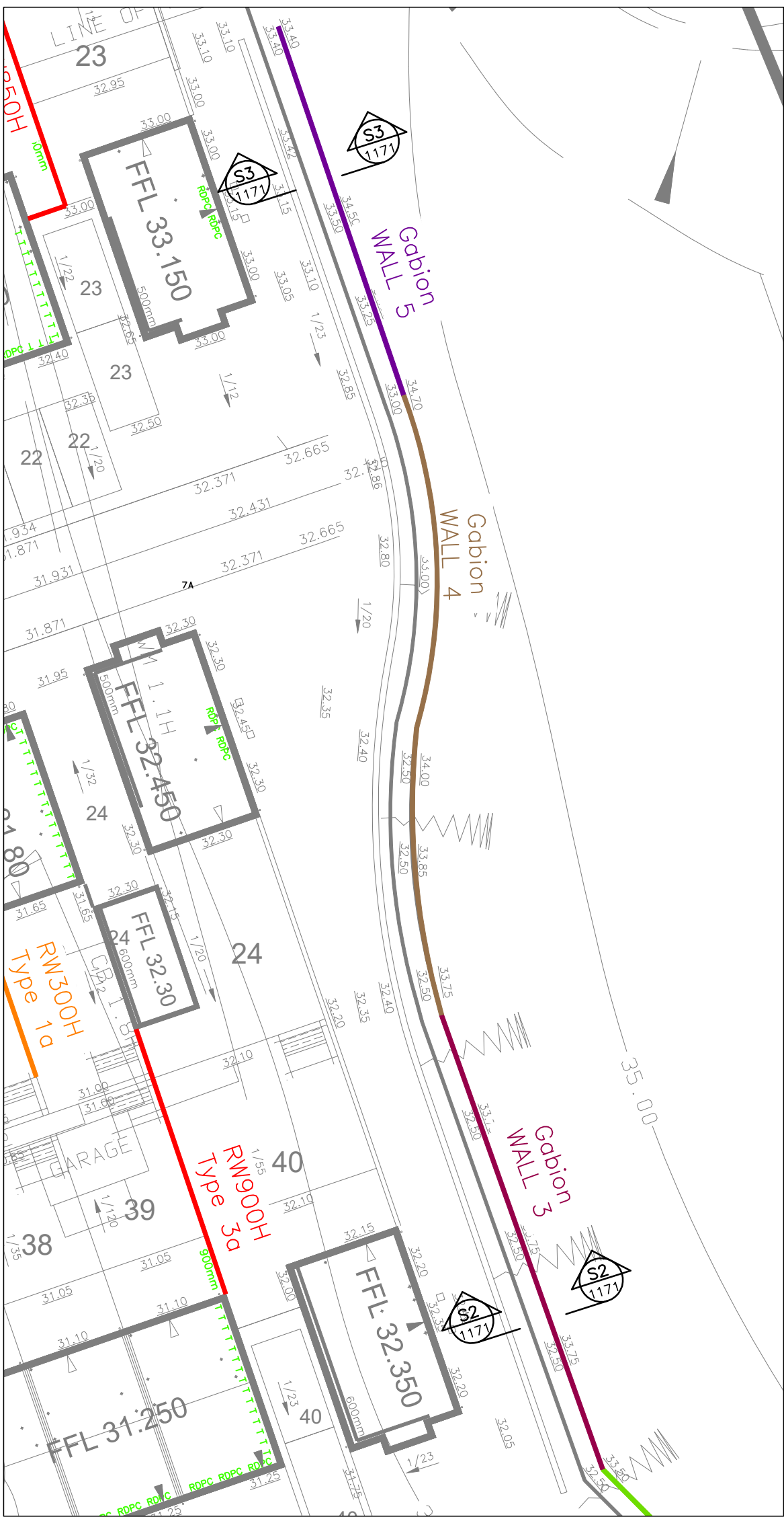
WALL'S 3,4 & 5 Location Plan (1:250)
