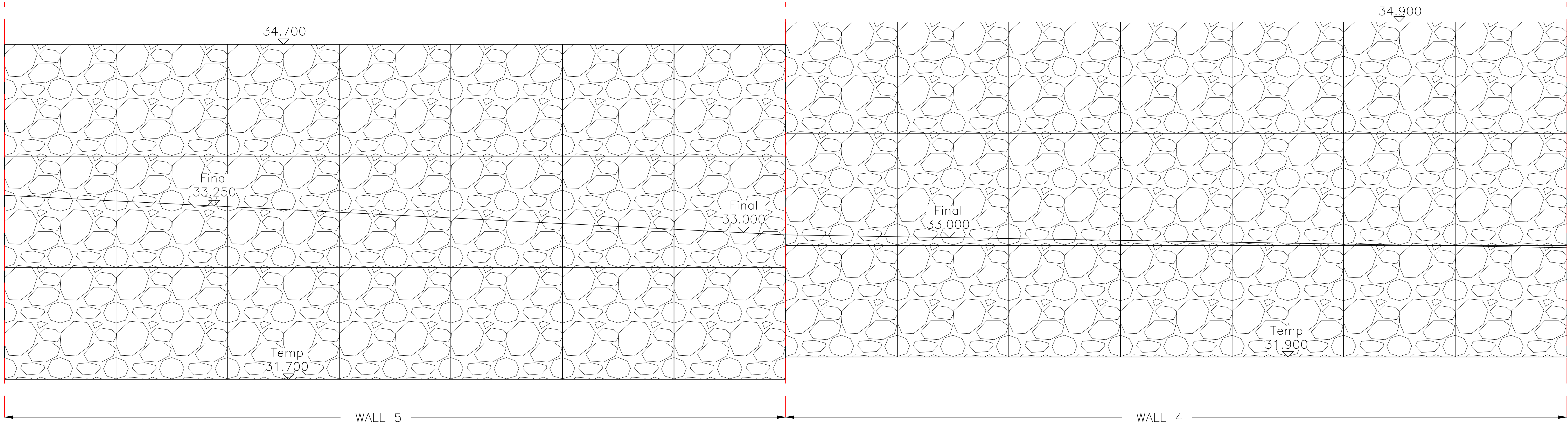
WALL 4 & 5 Woven Gabion Retaining Wall Elevation (1:20)
