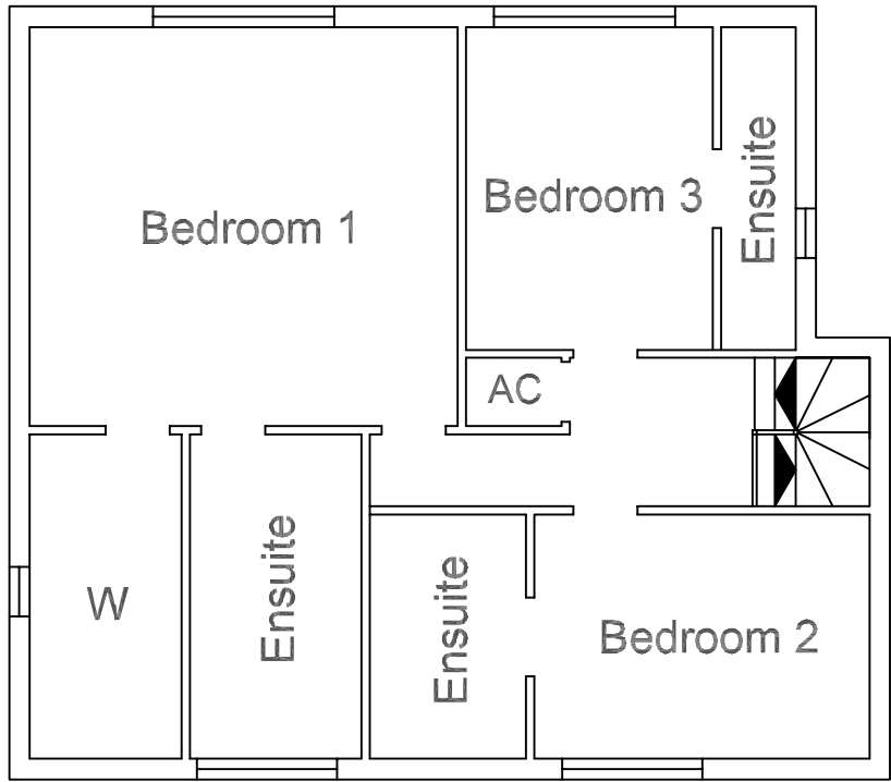
First Floor Existing
