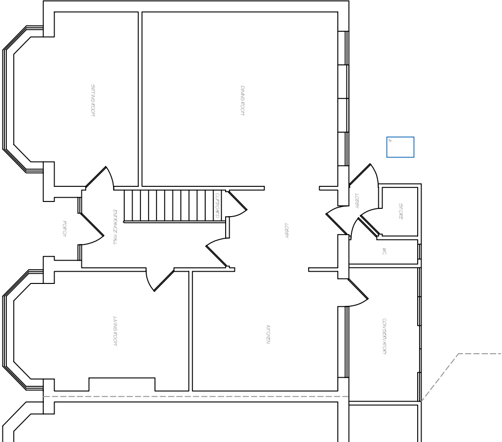
Existing Ground Floor Plan 1:100 @ A3
