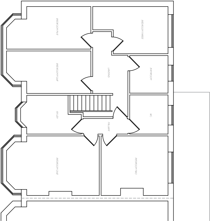
Existing First Floor Plan | : 1:00 @ A3
