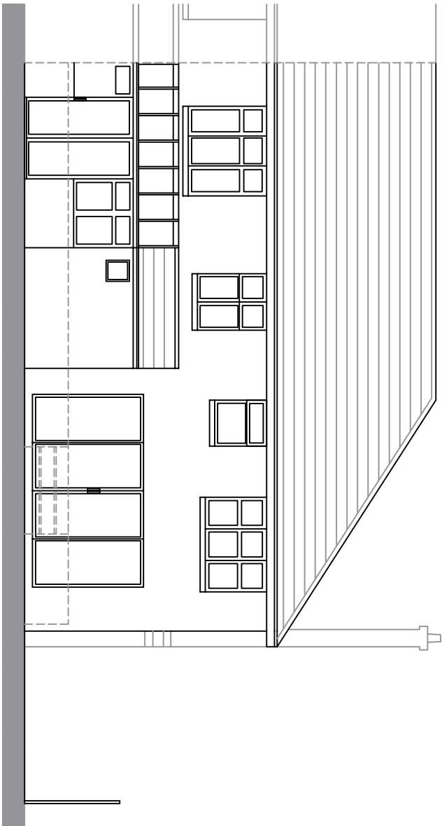
Existing Rear Elevation | : 1:00 @ A3
