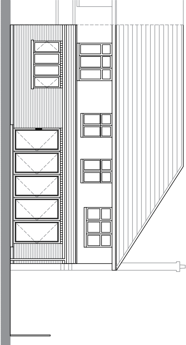
Proposed Rear Elevation | : 1:00 @ A3
