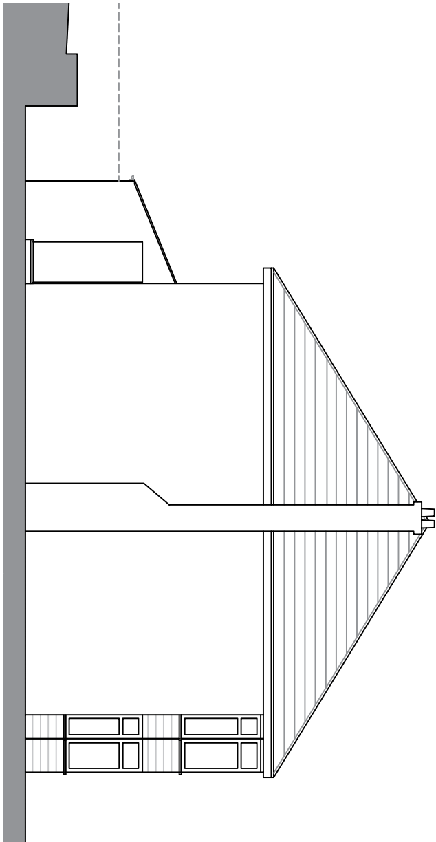
Existing Side Elevation | : 1:00 @ A3
