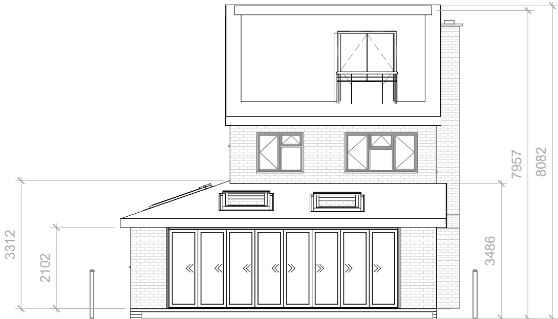
Proposed Elevation-Rear
