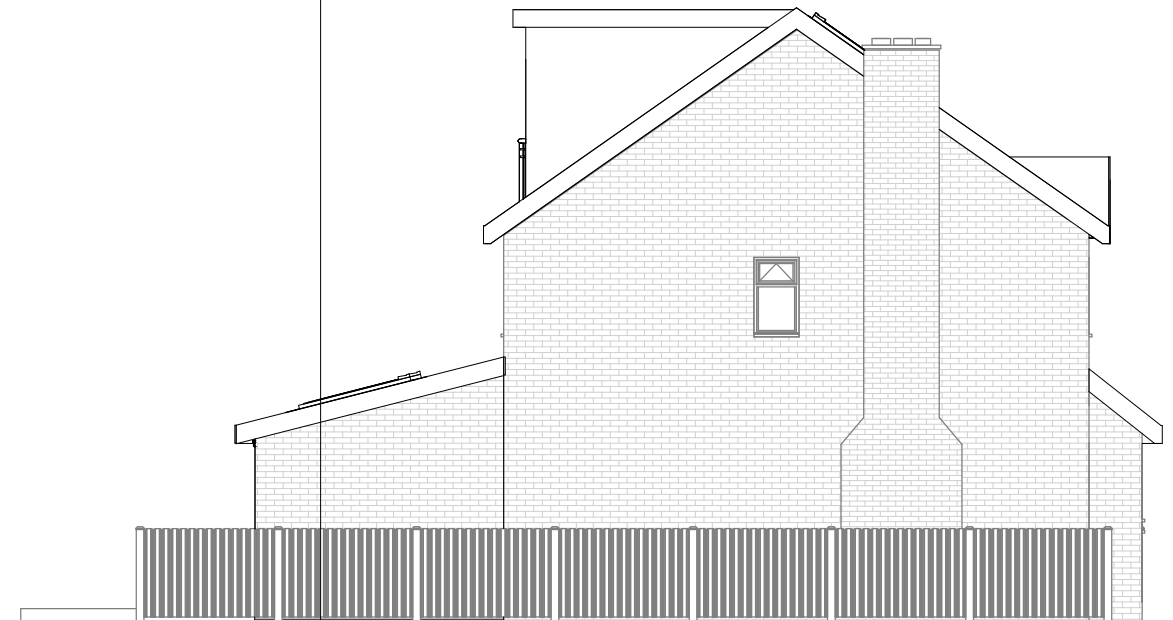
Proposed Elevation-Left side
