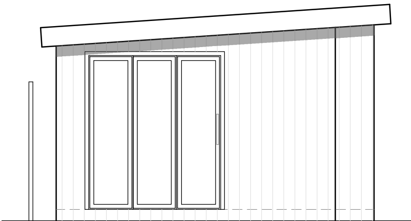
Proposed West Side Elevation - 1:50
