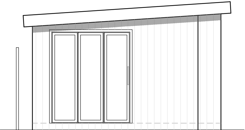
Proposed West Side Elevation - 1:50
