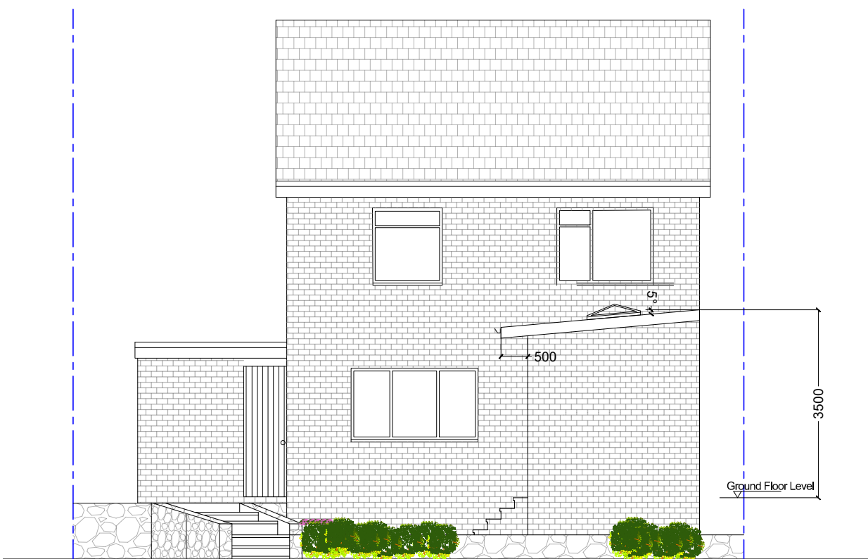
Proposed Rear Elevation 1:100 @A3
