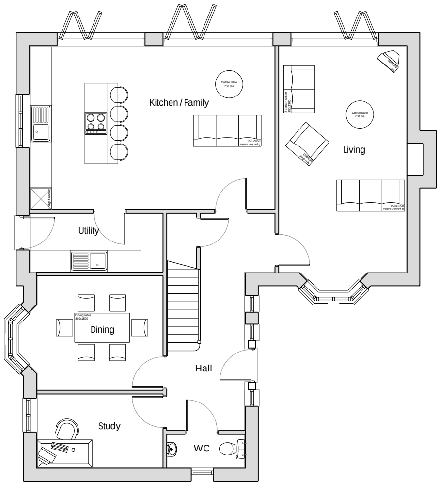
Ground Floor
