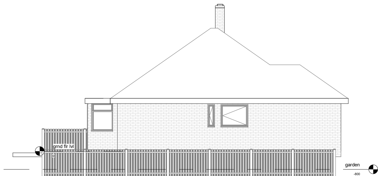
Existing Elevation-Left side
