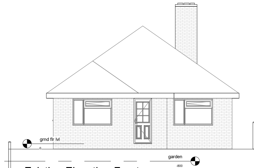
Existing Elevation-Front
