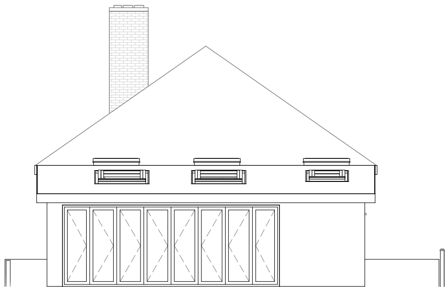
Proposed Elevation-Rear
