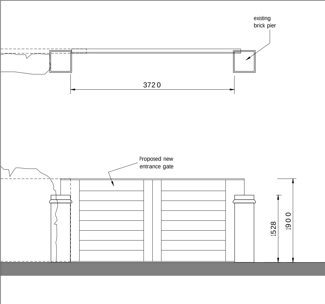
Proposed entrance gate
