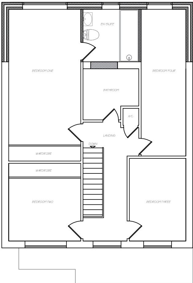
Proposed First Floor Plan 1:100 @ A3
