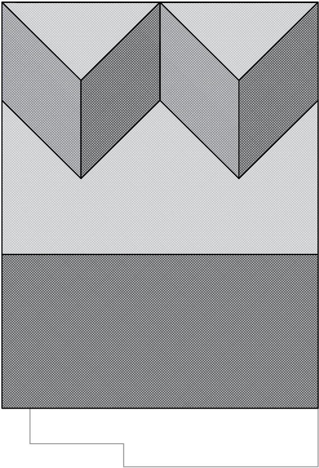
Proposed Roof Plan 1:100 @ A3
