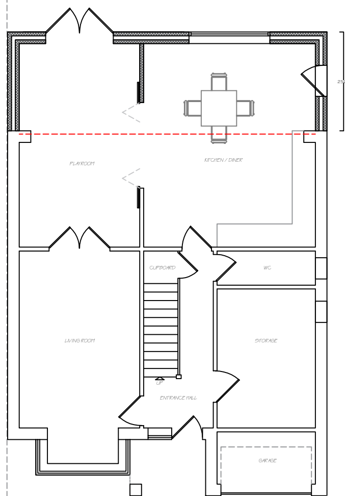
Proposed Ground Floor Plan 1:100 @ A3
