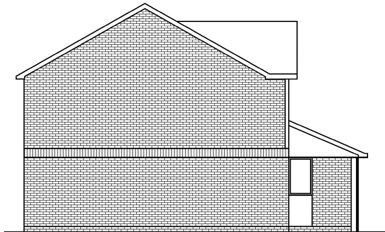
PROPOSED SIDE ELEVATION - EAST
