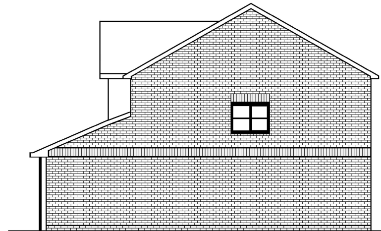
PROPOSED SIDE ELEVATION - WEST
