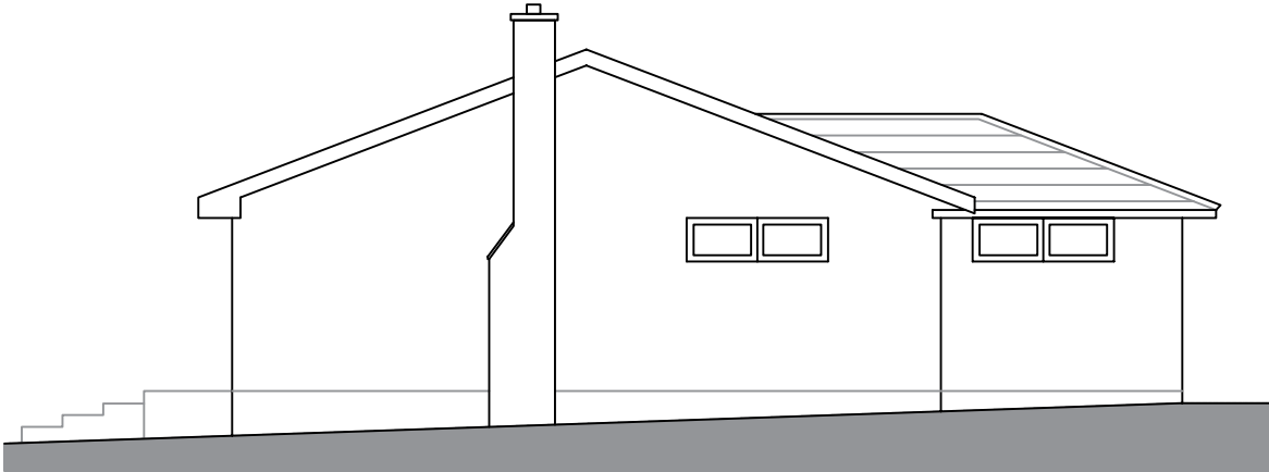
Existing Side Elevation 1:100 @ A3
