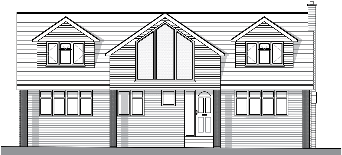
Proposed Front Elevation 1:100 @ A3
