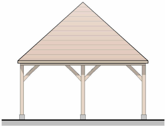
2 Rear Elevation - 1 : 100
