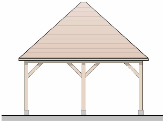
3 Side Elevation - 1 : 100
