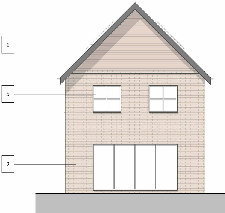
3 South West Elevation - 1 : 100
