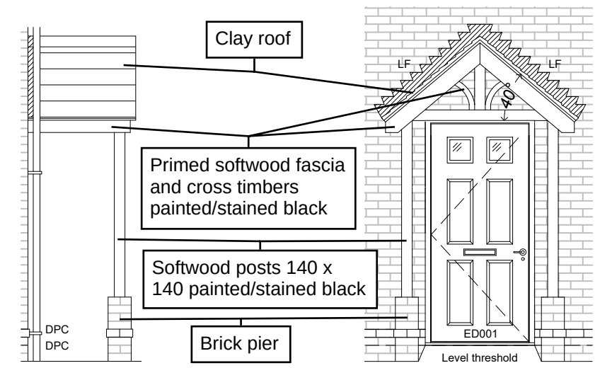
HT 5 Inner Housing Feature
