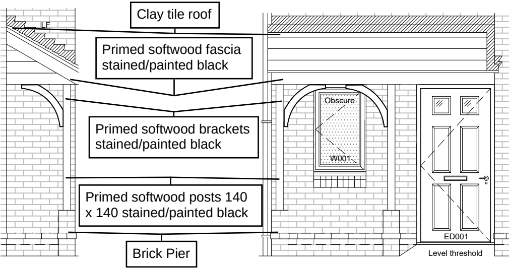
HT 3 Inner Housing Feature
