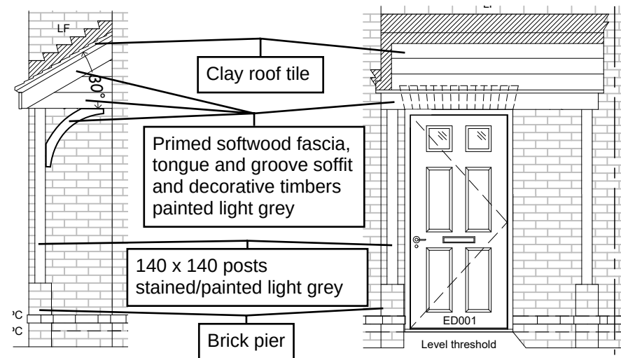
HT 7HA Inner Housing Please note side elevation not drawn so copied from HT 7
