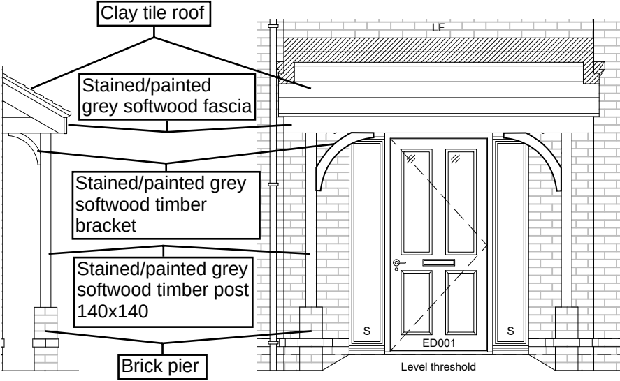
HT 1.1 Woodland Edge Feature
