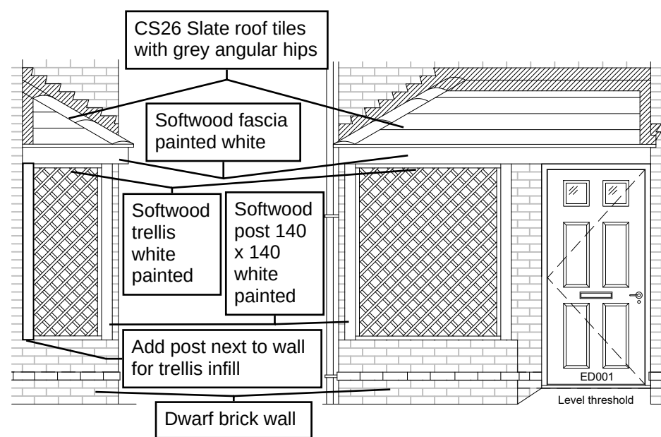
HT 3 Green Avenue & Green Avenue Feature
