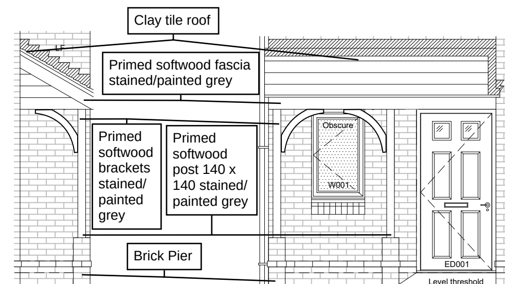
HT 3 Woodland Edge Feature
