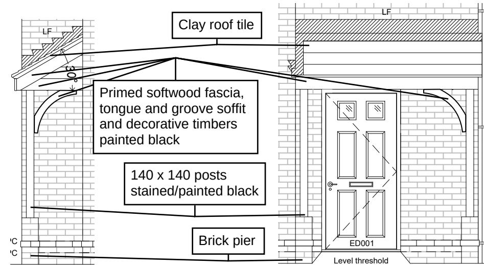
HT 7 Inner Housing Feature
