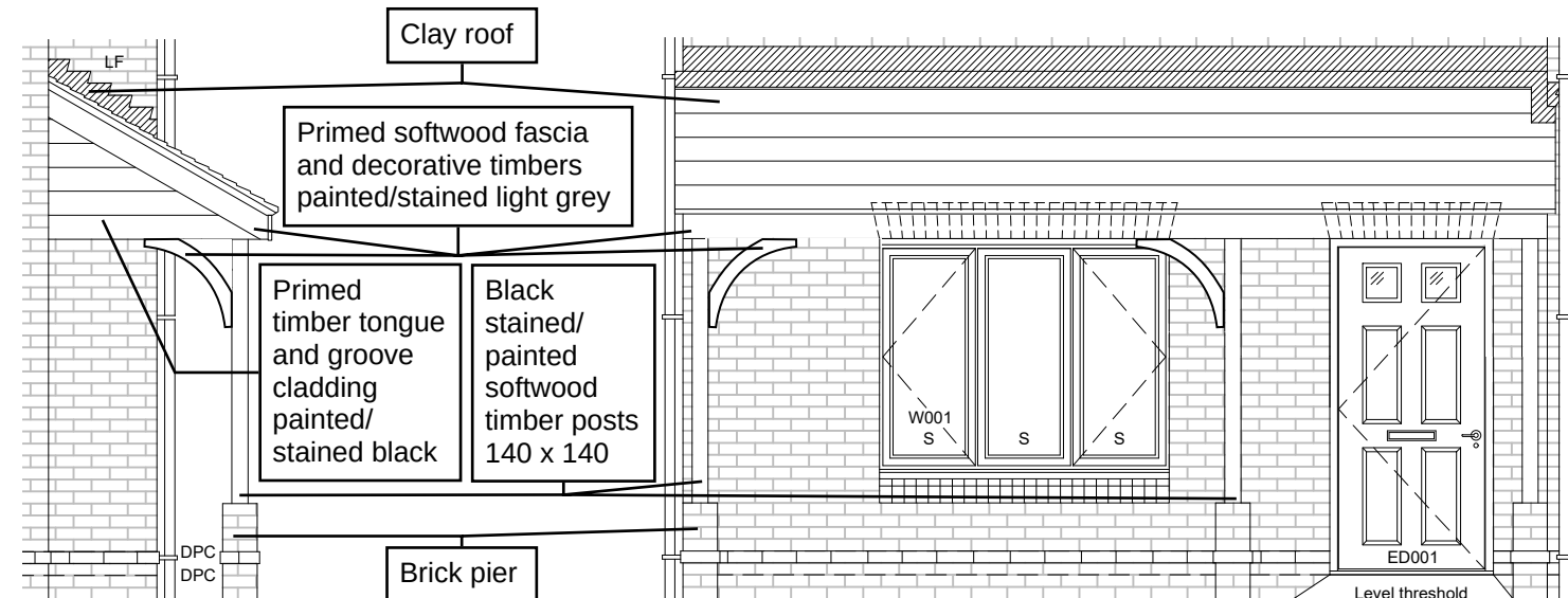
HT 6.2HA Inner Housing Feature
