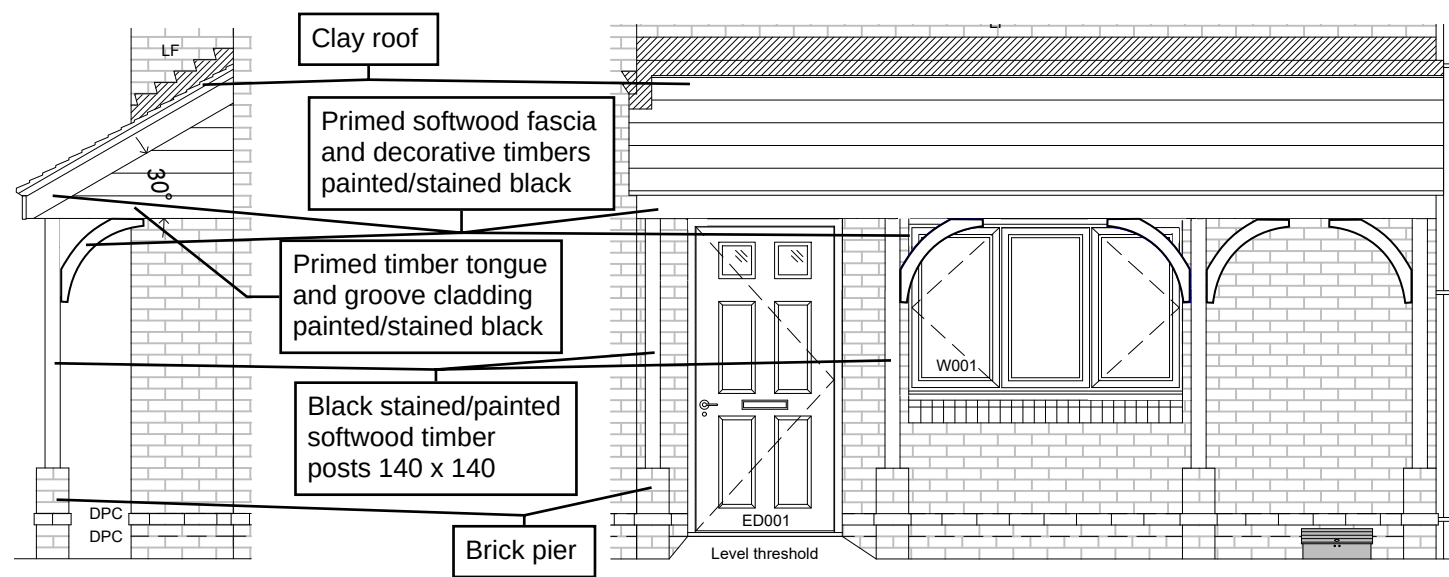
HT 6.2 Inner Housing Feature
