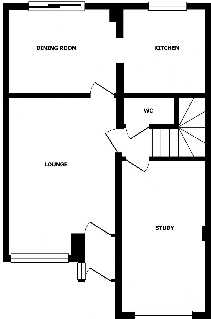
PROPOSED GROUND FLOOR LAYOUT PLAN
