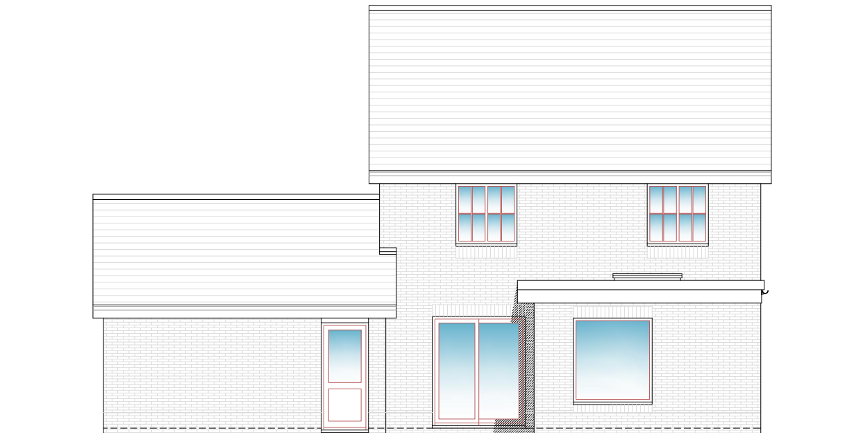
GREY GRP FLAT ROOF WHITE FASCIAS TO MATCH EXISTING WHITE UPVC RAINWATER GOODS TO MATCH EXISTING WHITE UPVC WINDOWS TO MATCH EXISTING WHITE ALUMINIUM DOORS TO MATCH EXISTING
