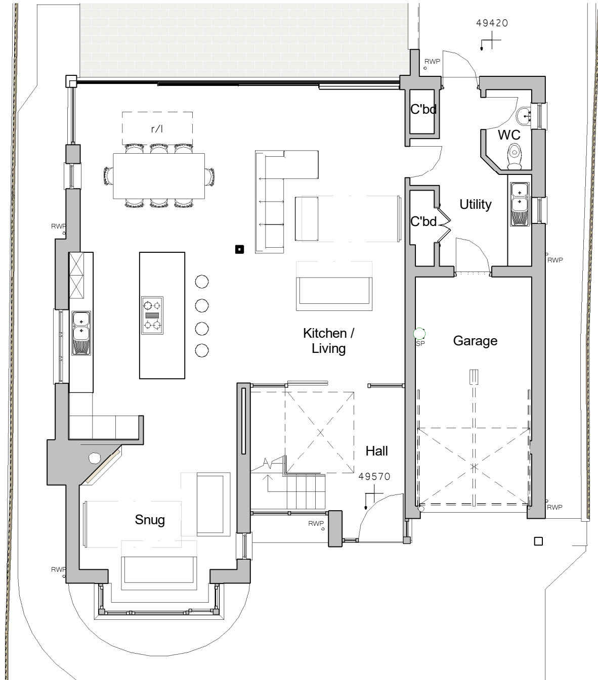
Ground Floor Plan as Proposed 1 : 100
